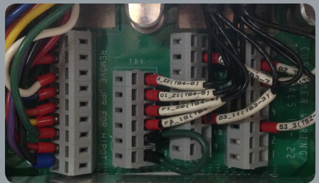
Wiring behind front panel through glands (P3)
